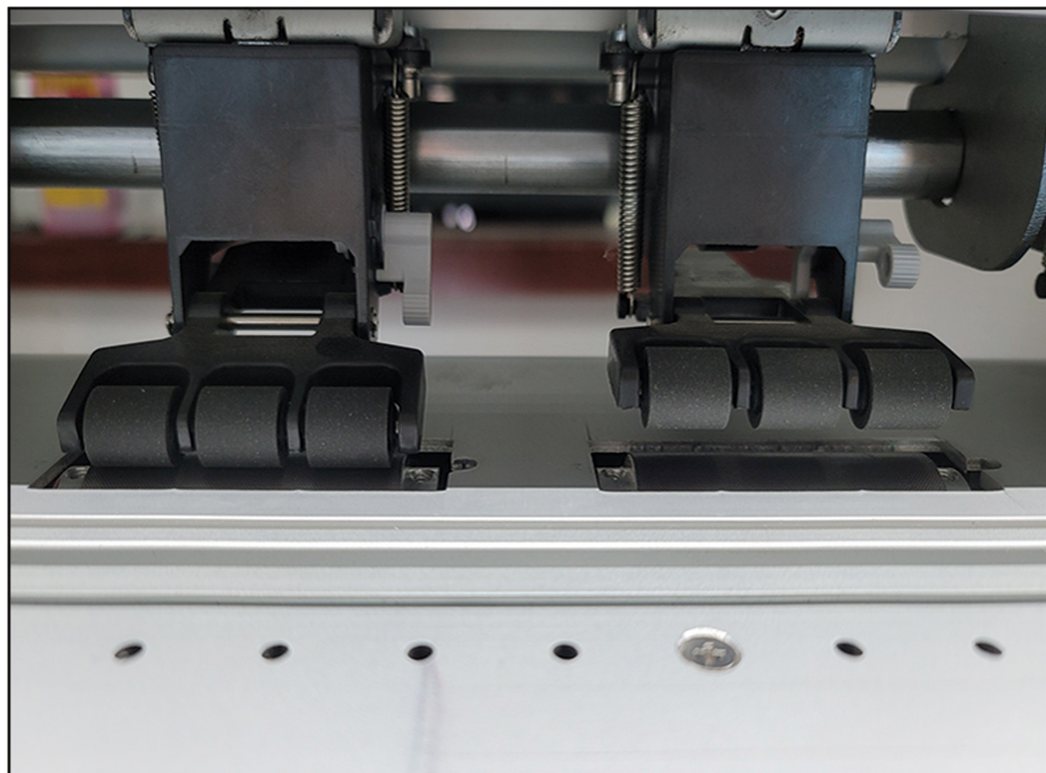
Individually Operating Pinch Roller
