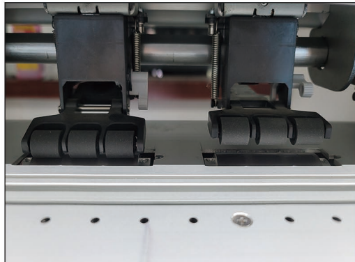
Individually Operating Pinch Roller
