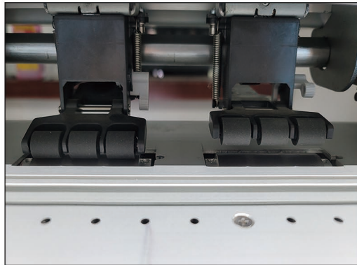
Individually Operating Pinch Roller
